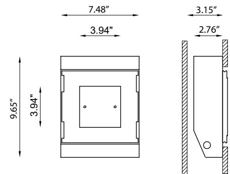
Fixture Dimensions
