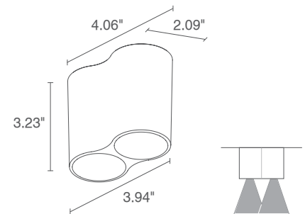
Fixture Dimensions
