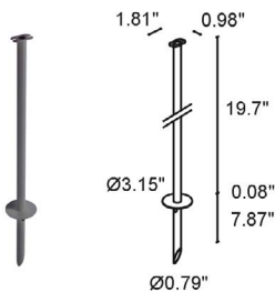
WP1006 __ (Length 19.69") WP1007 __ (Length 31.50") Ground Spike with Bracket Include one of the below finishes: I - Stainless Steel E - White F - Gray H - Anthracite T - Cor-ten 5 - Jasper Green C - Custom RAL
