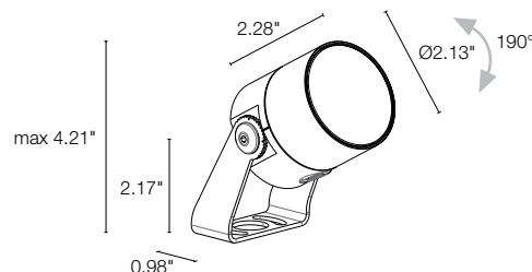
Fixture Dimensions
