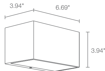
Fixture Dimensions
