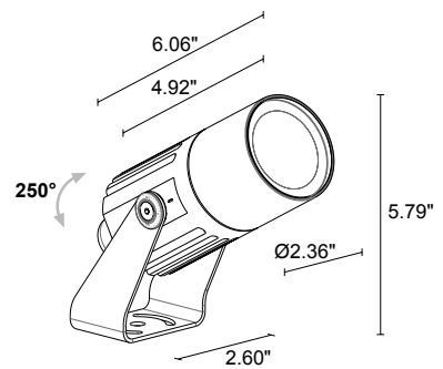
Fixture Dimensions
