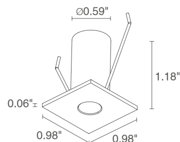
Ceiling Cut-Out: Ø 0.71" Fixture Dimensions
