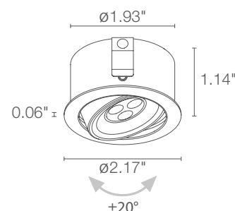
Ceiling Cut-Out: \varnothing 1.97" Fixture Dimensions
