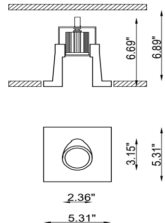
Fixture Dimensions
