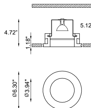
Fixture Dimensions
