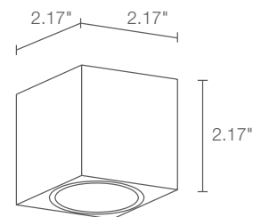
Fixture Dimensions
