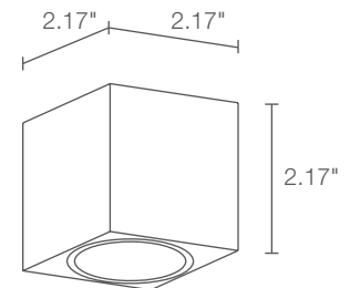
Fixture Dimensions
