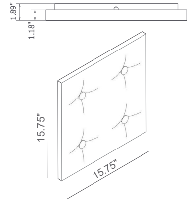
Fixture Dimensions
