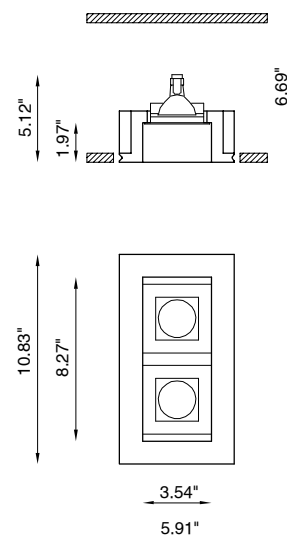
Fixture Dimensions
