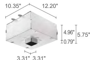
WC8701 Outer casing for rebated installation in solid ceilings (Bitpop 2.2)
