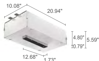
WC8709 Outer casing for rebated installation in solid ceilings (Bitpop 8.1)
