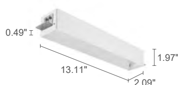
WC8710 - White WC8710N - Black Outer casing for deep-set installation in plasterboard ceilings (Bitpop 8.1)
