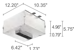
WC8702 Outer casing for rebated installation in solid ceilings (Bitpop 4.1)
