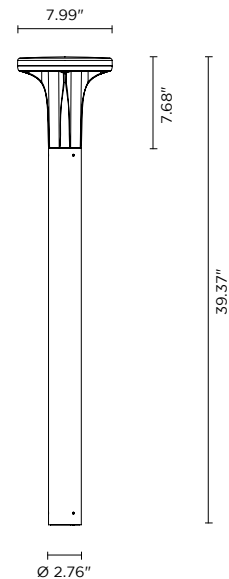
Fixture Dimensions:
