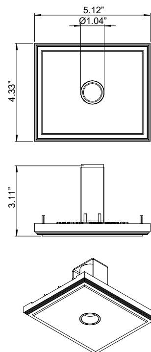
Fixture Dimensions
